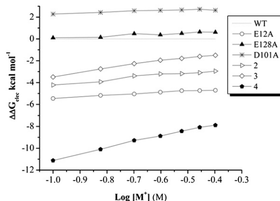
FIGURE 7 \Delta\Delta G_{\text{elec}} (kcal mol -1 ) versus the logarithm of salt concentration (1:1 salt, in M). The calculations are based on the nonlinear solution to the Poisson-Boltzmann equation. The wild-type PwTBP is set as the reference energy. Mutants E12AE128A, E12AE42KE138A, and E12AD41KE42KE128A are labeled 2, 3, and 4, respectively.
