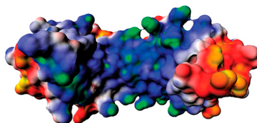
FIGURE 9 Electrostatic potential map for the Pw TBP quadruple mutant protein. The electrostatic potential ranges from -2 \text{ kT/e} to +2 \text{ kT/e} : yellow-red, negative; white, neutral; and blue-green, positive. The orientation of the quadruple-mutant Pw TBP is the same as in Fig. 1 A.
